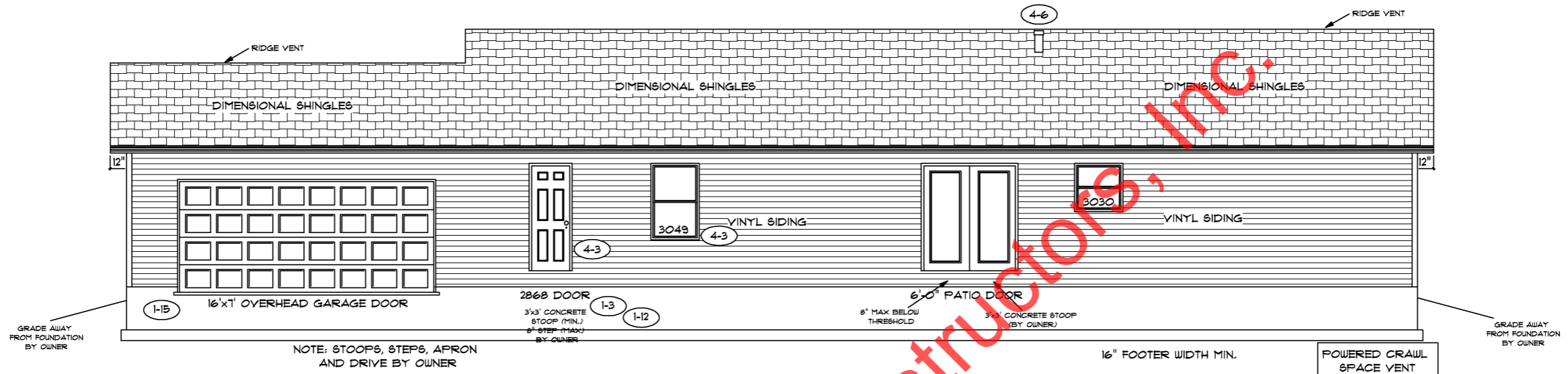
REAR ELEVATION
