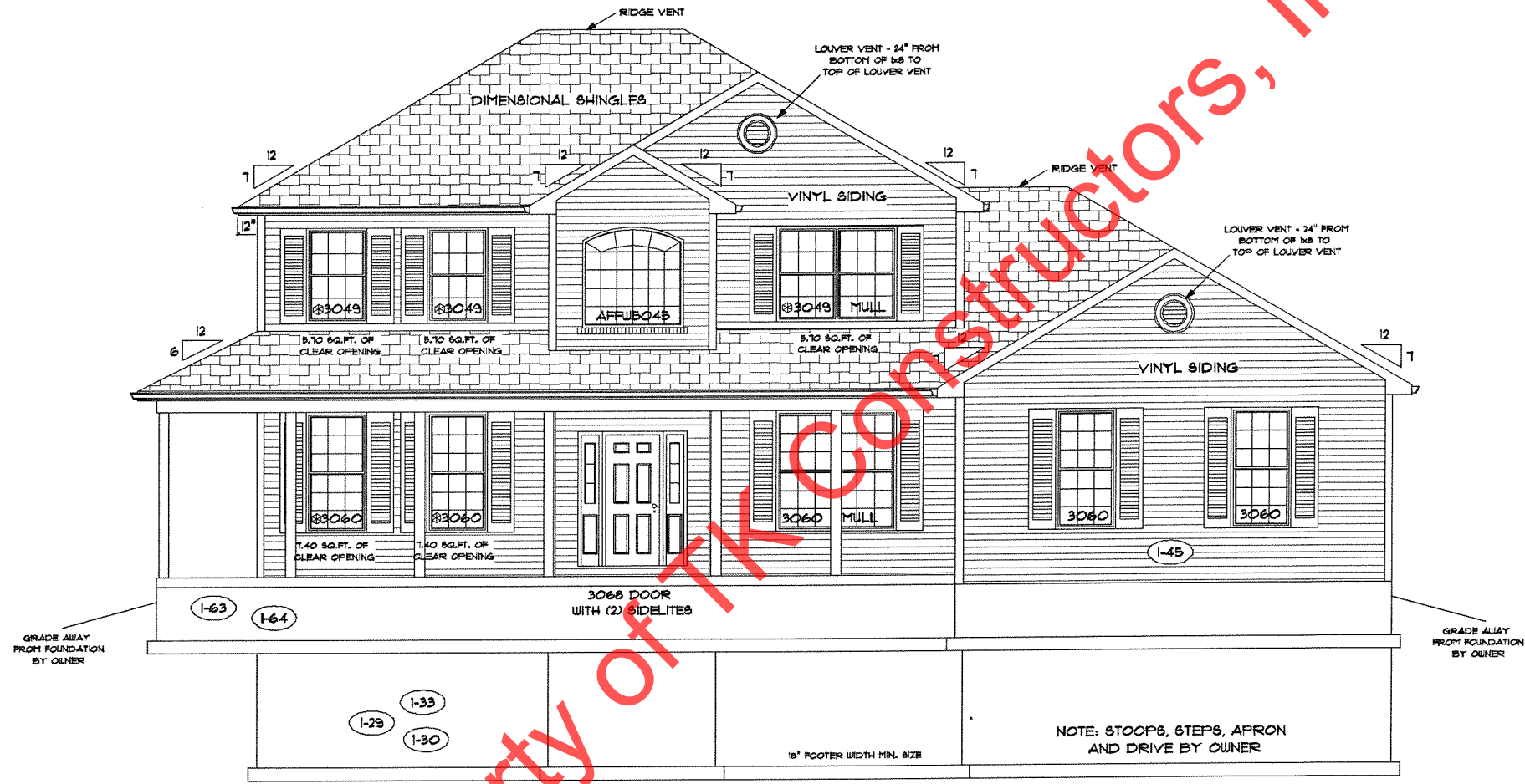
FRONT ELEVATION
