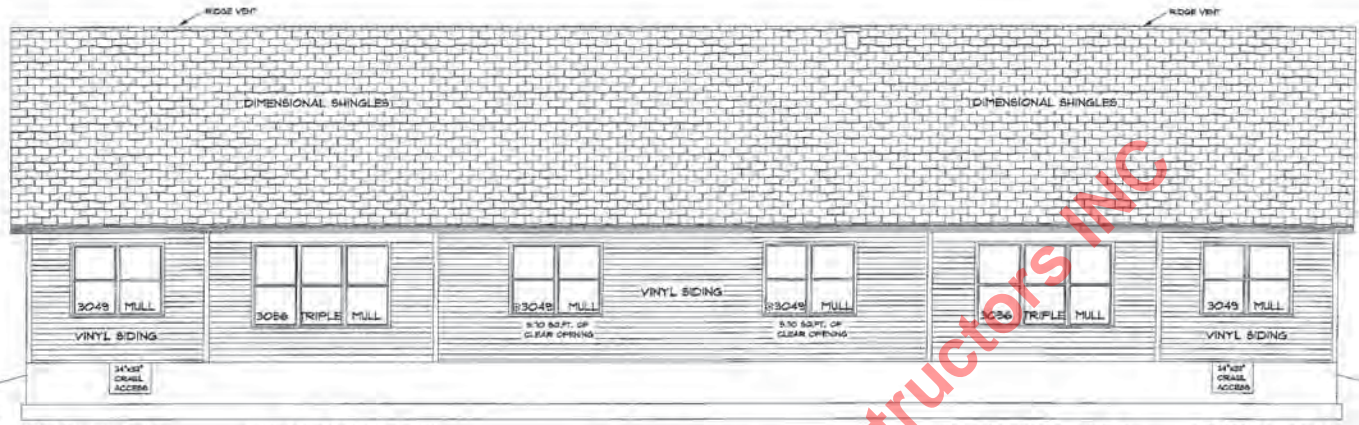
REAR ELEVATION
