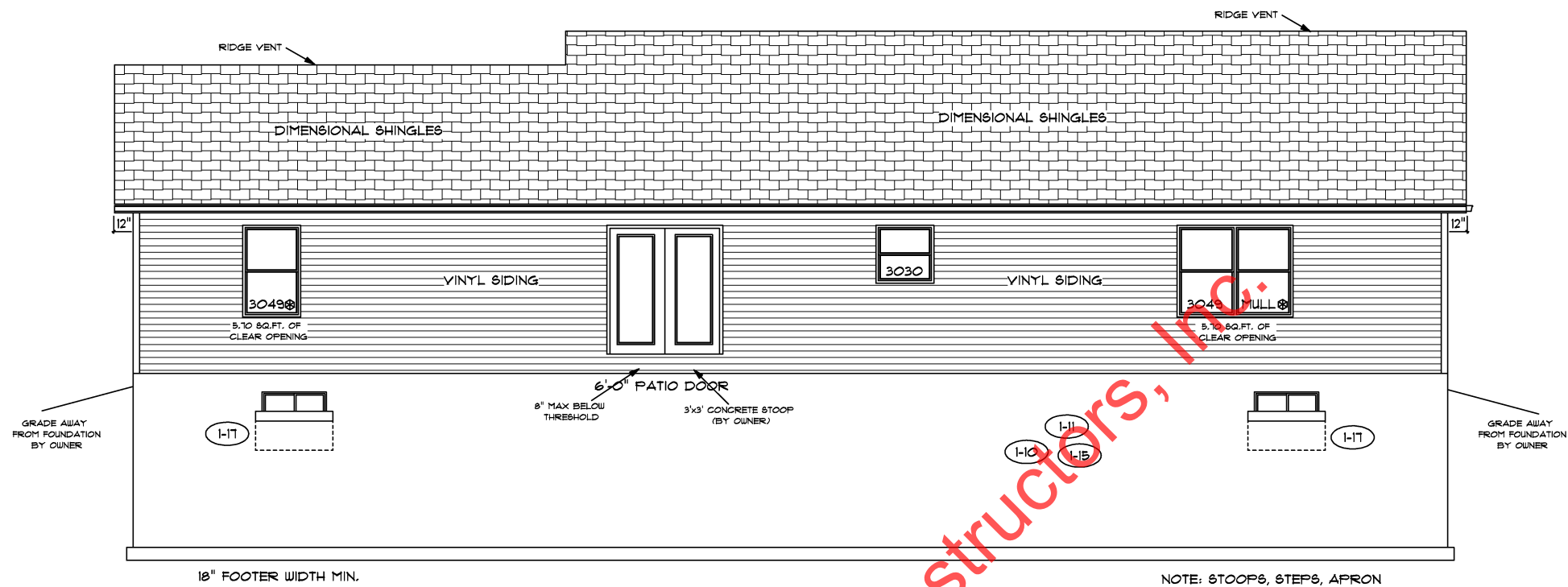
REAR ELEVATION
