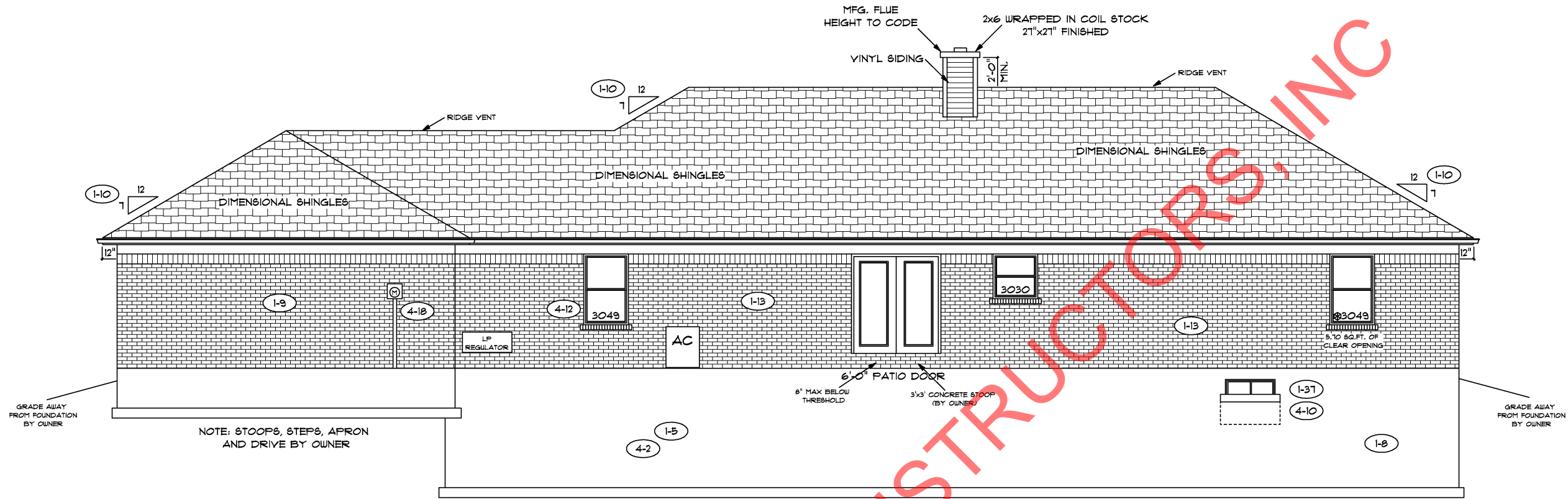
REAR ELEVATION
