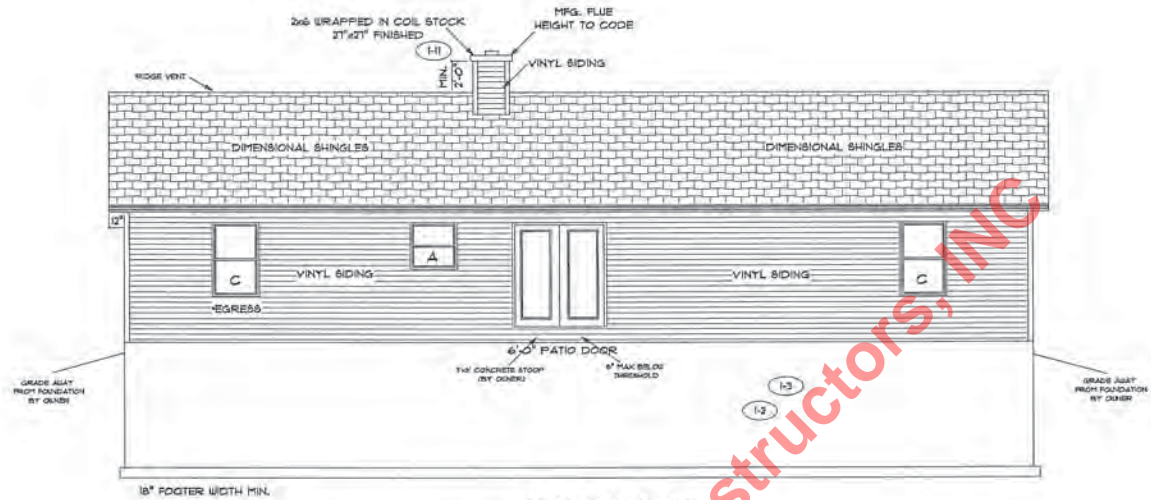
REAR ELEVATION
