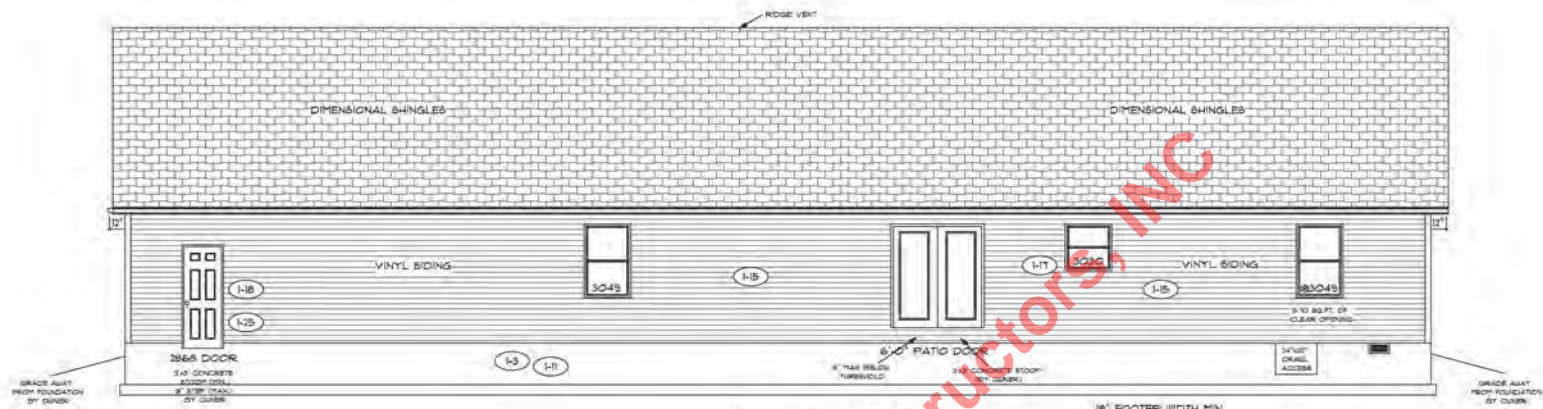
REAR ELEVATION
