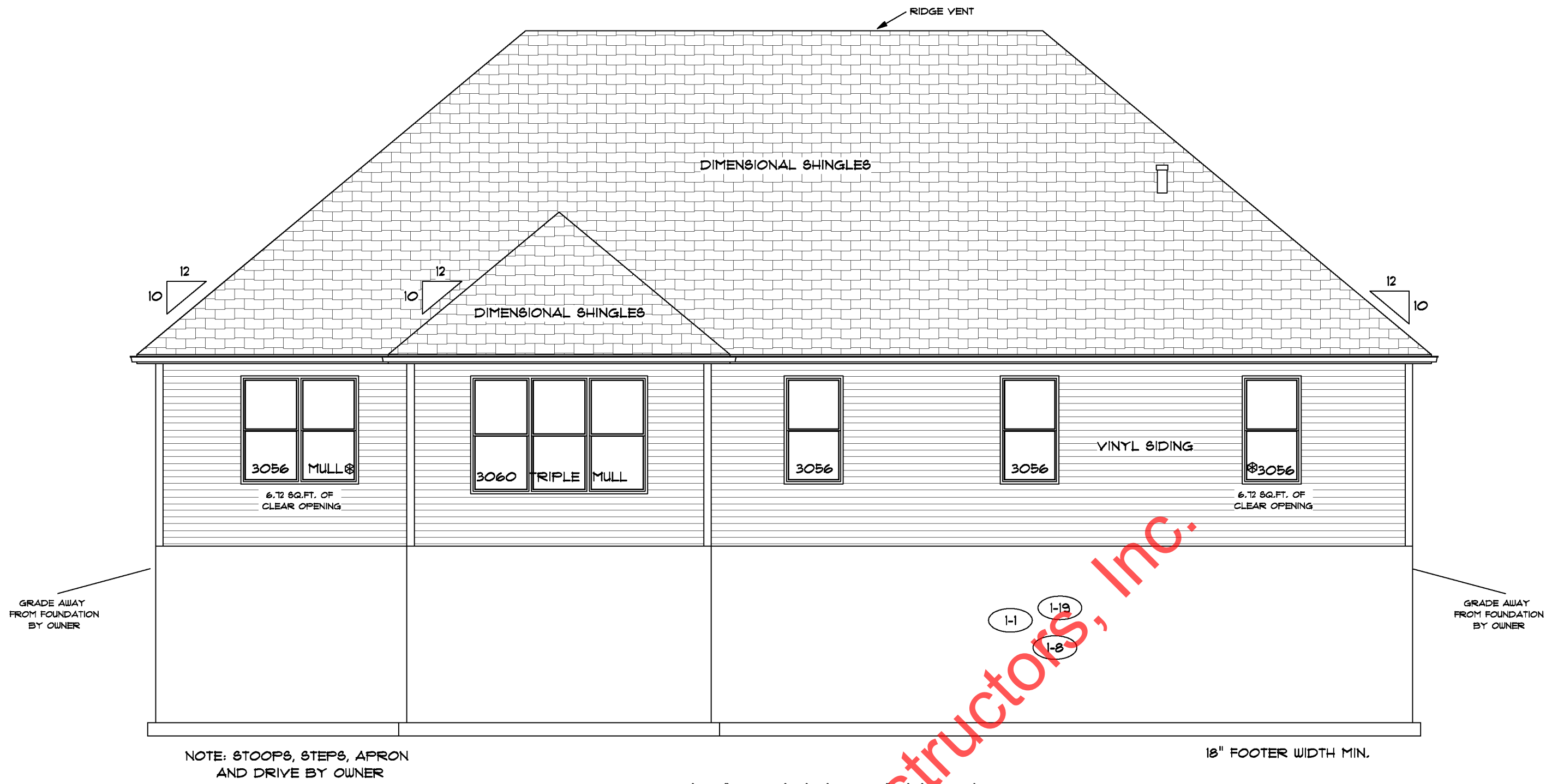
REAR ELEVATION
