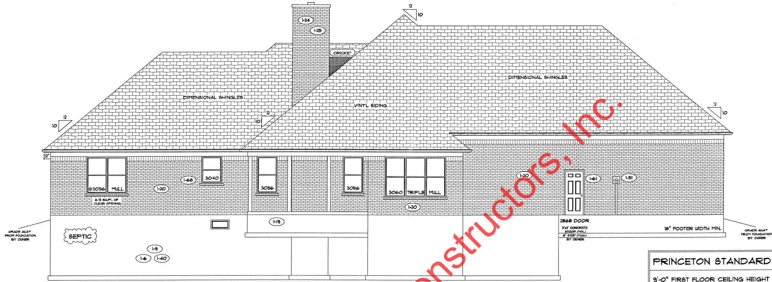
REAR ELEVATION
