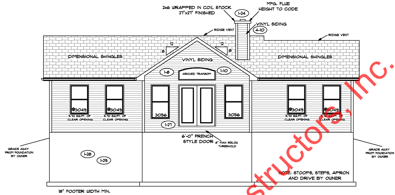
REAR ELEVATION
