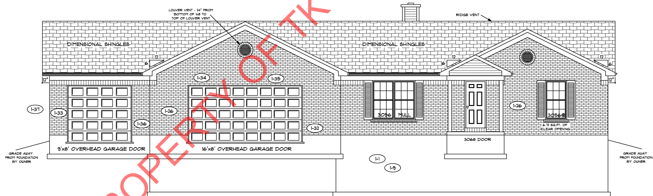
FRONT ELEVATION
