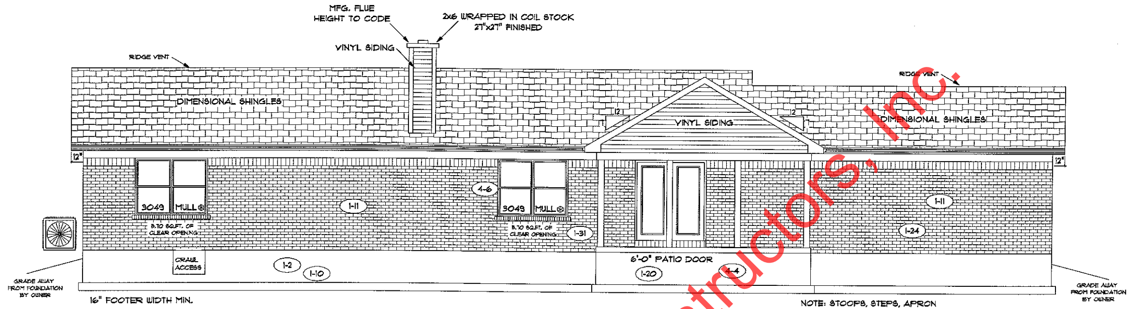
REAR ELEVATION
