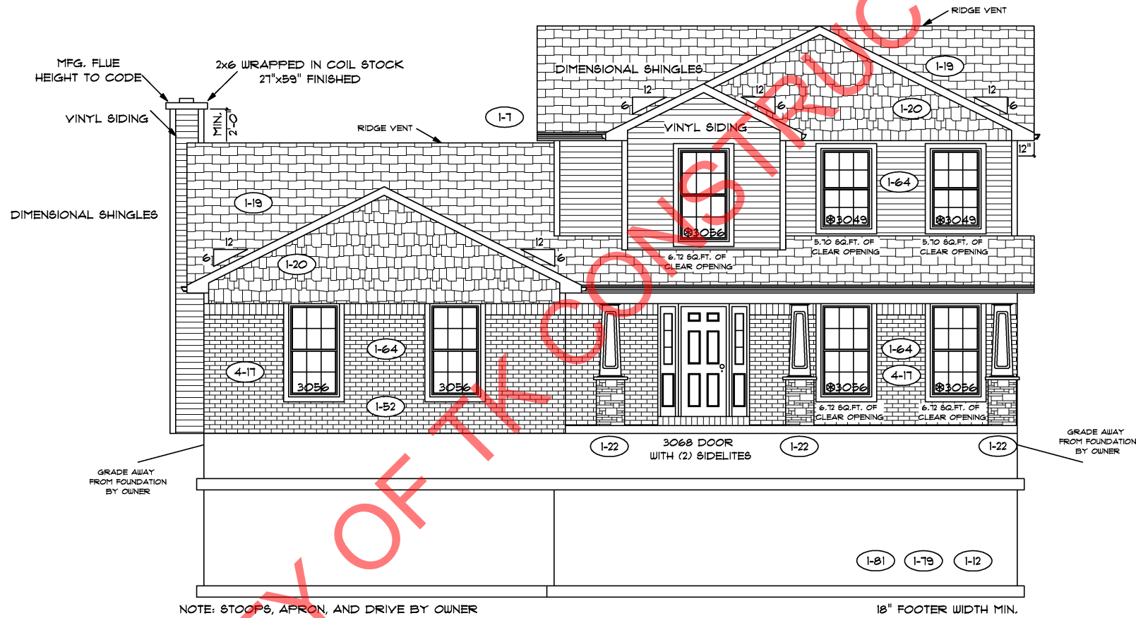
FRONT ELEVATION
