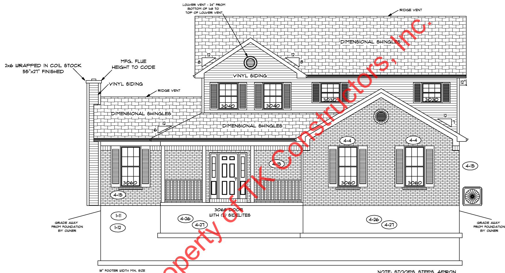
FRONT ELEVATION
