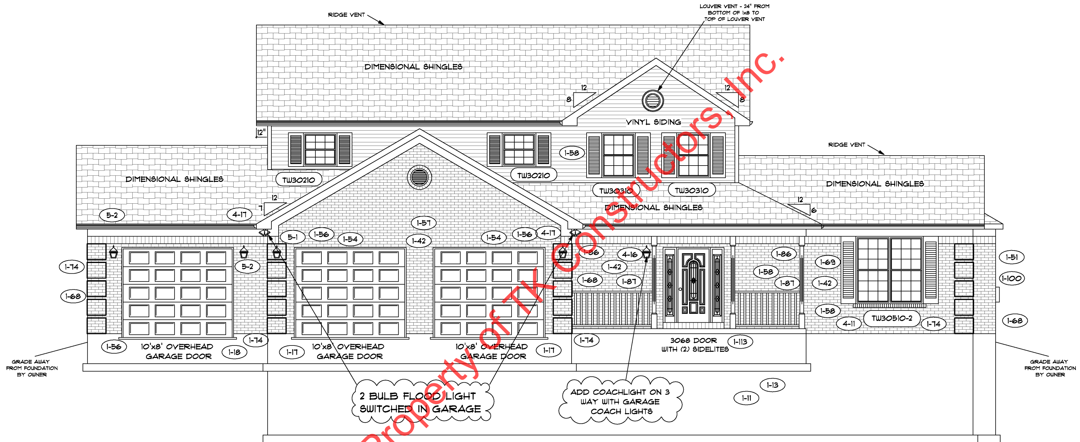
FRONT ELEVATION
